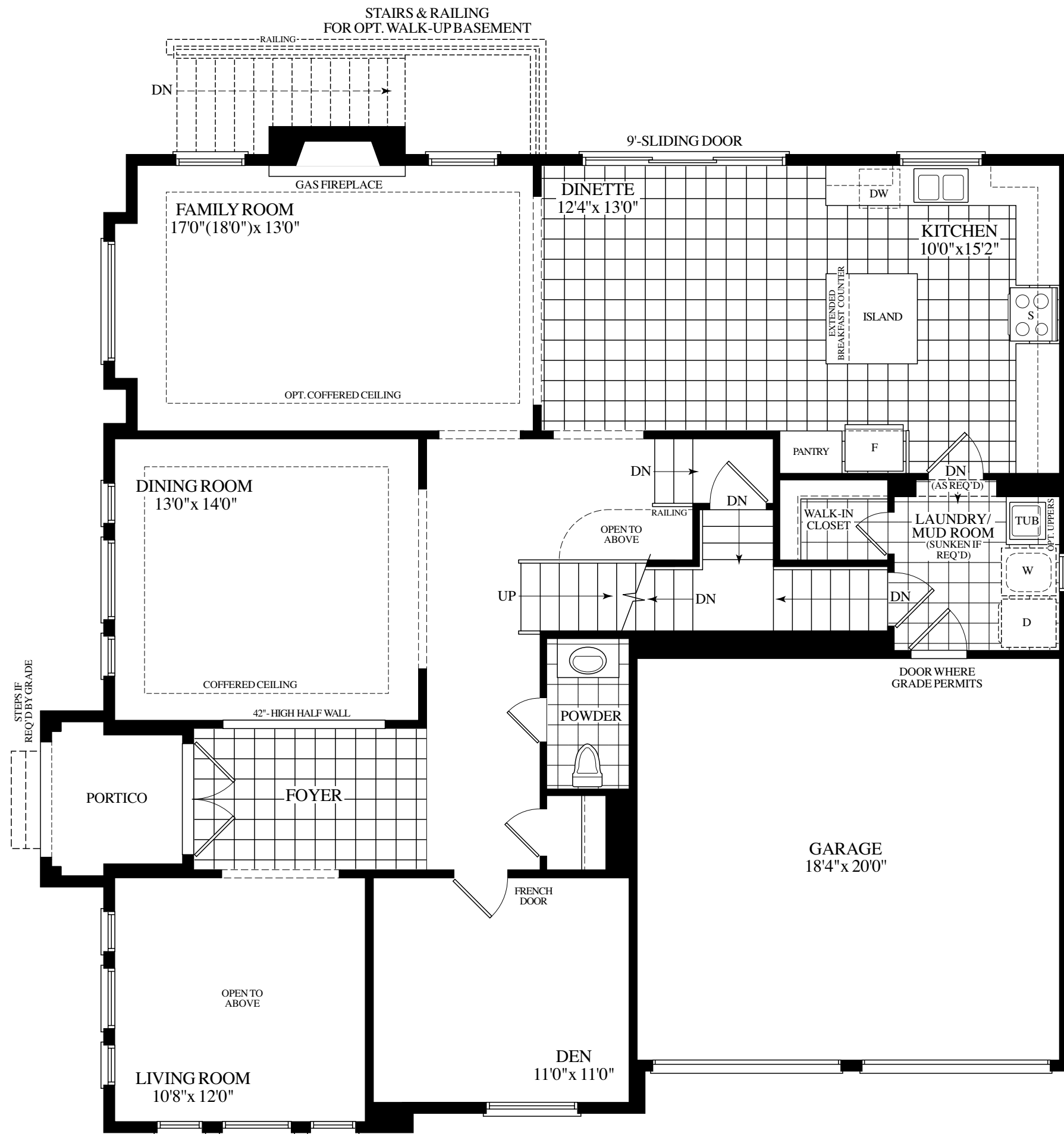
MAIN LEVEL ELEV. A
