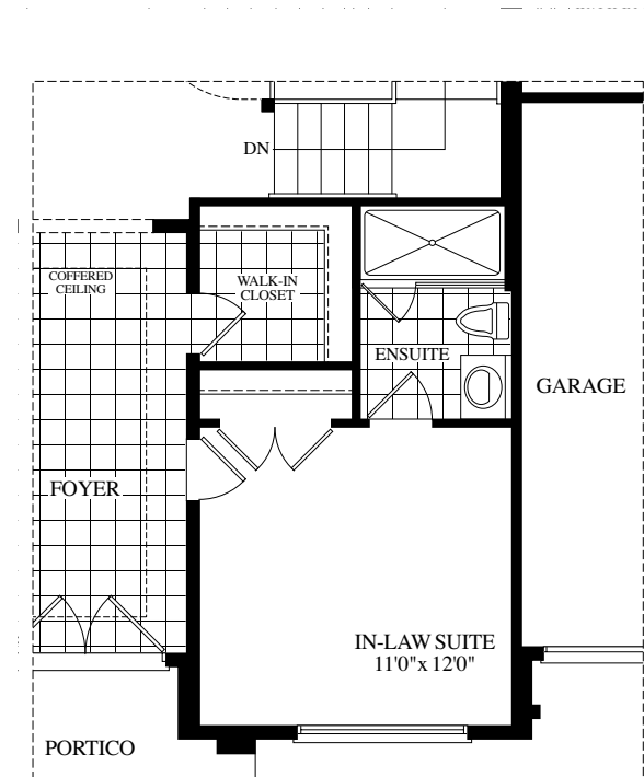
PART MAIN LEVEL WITH OPT. IN-LAW SUITE ELEV. A (ELEV. B - SIMILAR)
