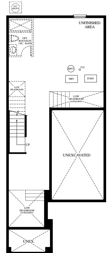
LOWER LEVEL ELEVATION A & B
