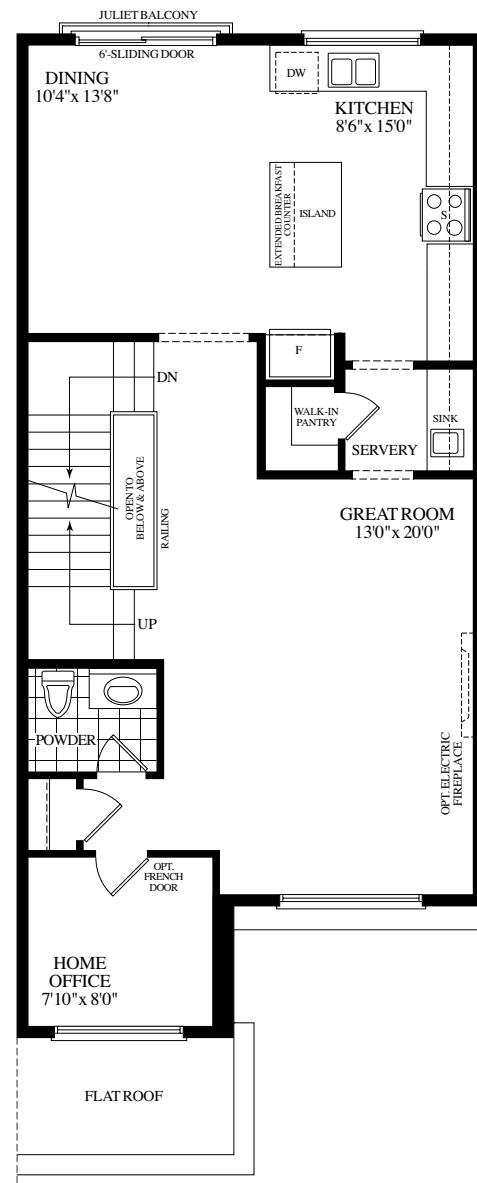
MAIN LEVEL ELEVATION A & B
