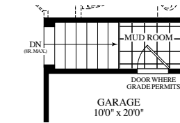
GROUND LEVEL ELEVATION A & B (8 RISERS SUNKEN CONDITION)
