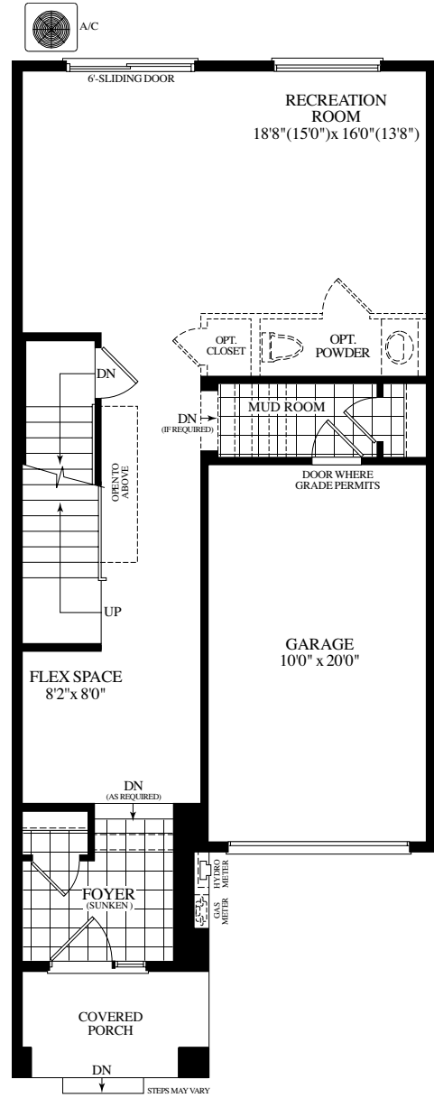
GROUND LEVEL ELEVATION A & B
