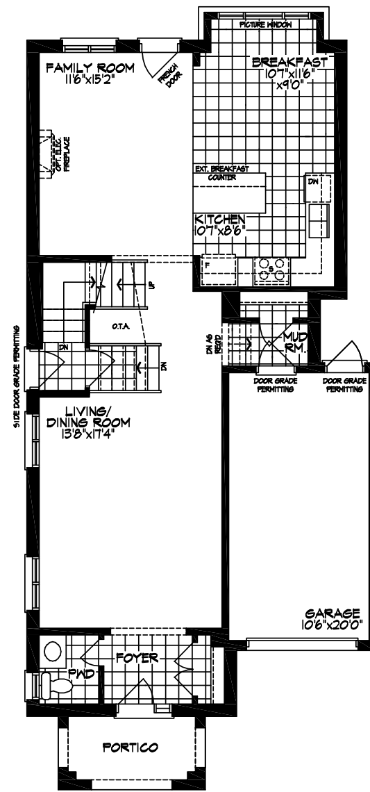
GROUND FLOOR ELEVATION A1 & A2 (REV)
