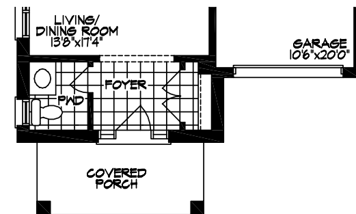
GROUND FLOOR ELEVATION B1 & B2 (REV)
