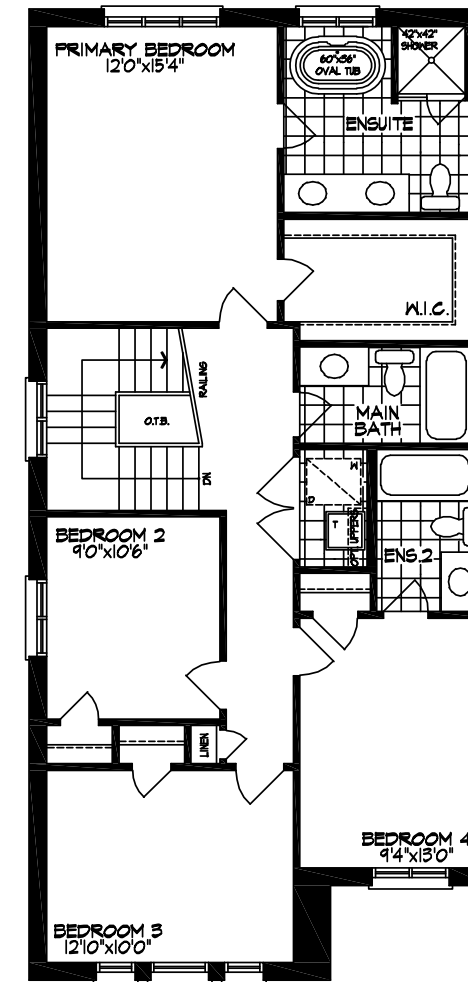
OPT. SECOND FLOOR W/4 BEDROOMS & 3 BATHROOMS ELEVATION A1 & A2 (REV)
