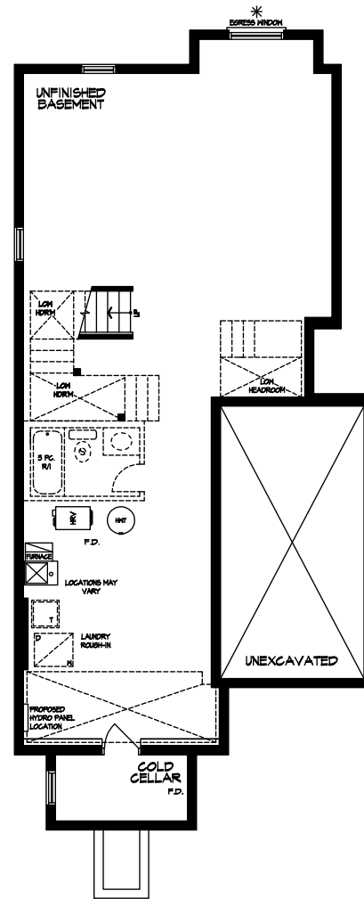
BASEMENT ELEVATION A1 & A2 (REV)
