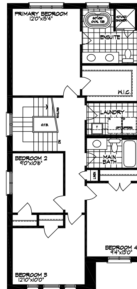
OPT. SECOND FLOOR W/4 BEDROOMS ELEVATION A1 & A2 (REV)
