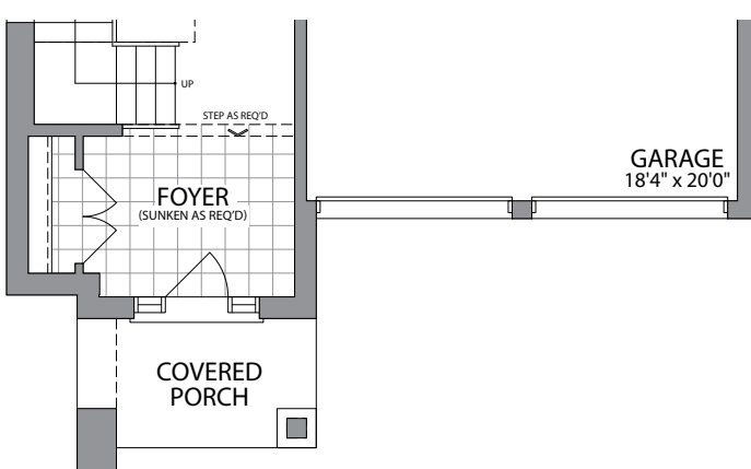
GROUND FLOOR ELEV. C
