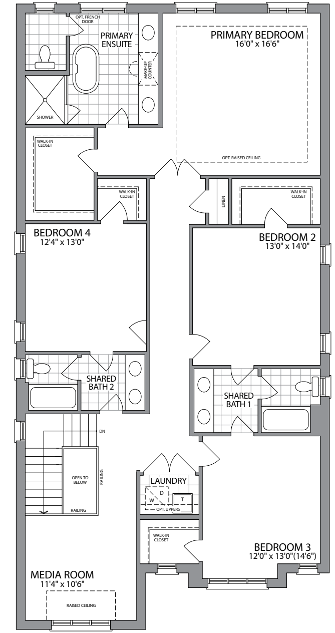
OPT. SECOND FLOOR W/LAUNDRY & MEDIA ROOM ELEV. A
