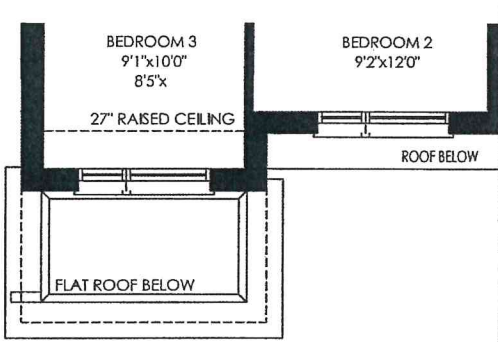
SECOND FLOOR PLAN, EL. 'B'
