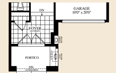
MAIN LEVEL ELEVATION C
