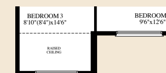
OPT. UPPER LEVEL W/3 BATHROOMS ELEVATION B
