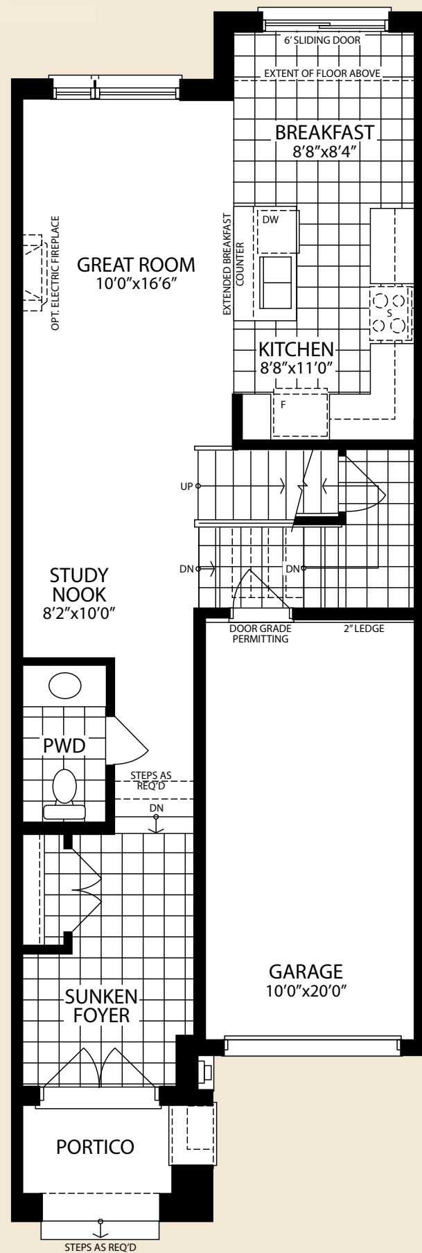
MAIN LEVEL W/STUDY NOOK ELEVATION A
