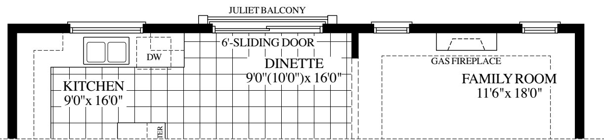
PART MAIN LEVEL - LOT 115 (WALK-OUT CONDITION)
