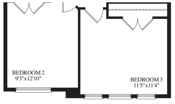
UPPER LEVEL ELEV. A2
