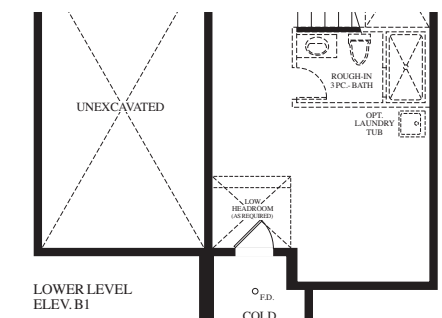
LOWER LEVEL ELEV. B1
