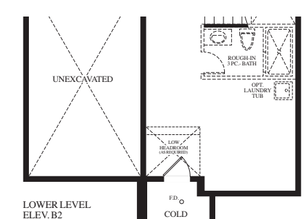
LOWER LEVEL ELEV. B2
