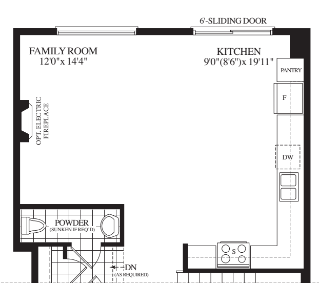
PARTIAL MAIN LEVEL WITH OPT. KITCHEN LAYOUT ELEV. A1, A2, B1 & B2
