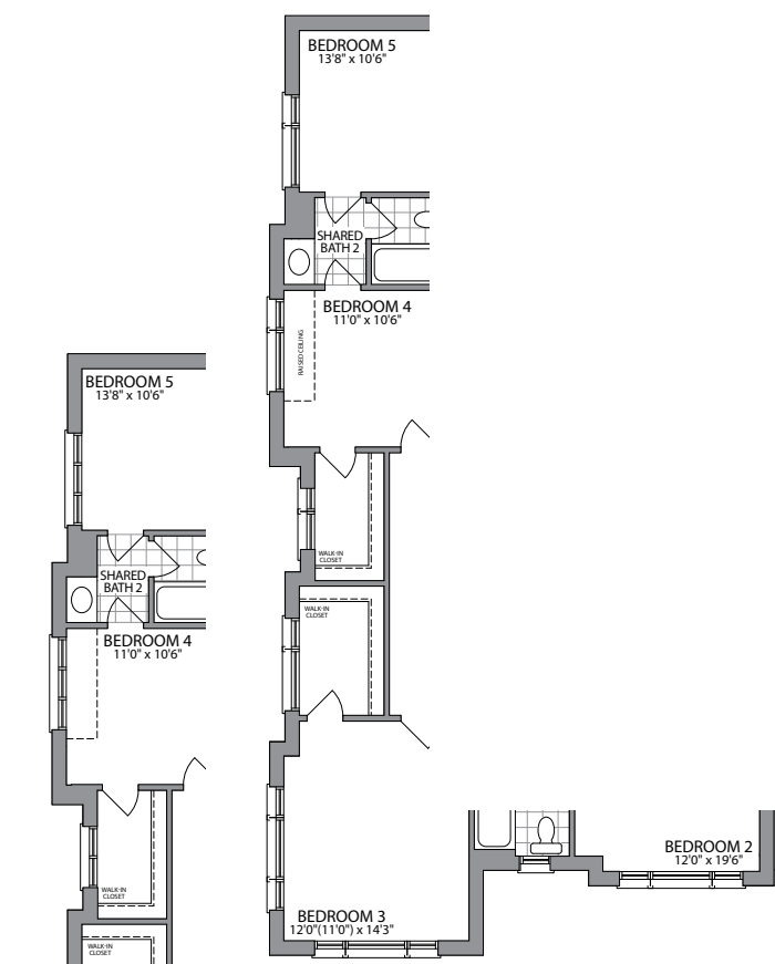
OPT. SECOND FLOOR ELEV. C
